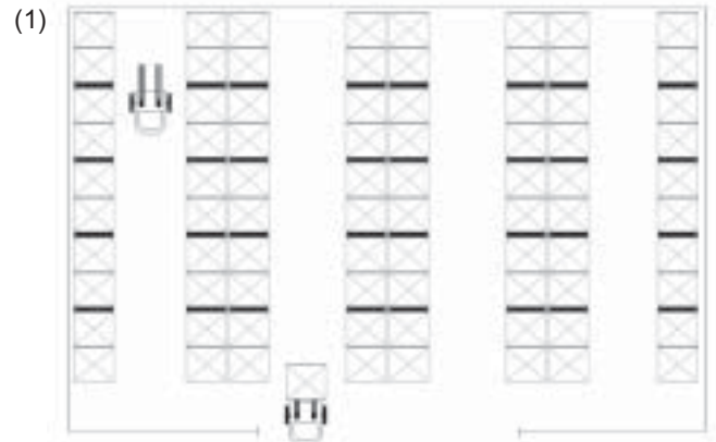
Top view of selective pallet rack warehouse. The forklift has access to rows of pallet rack on both sides.
